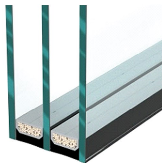
Double glazing (single chamber) Triple glazing (double chamber)
